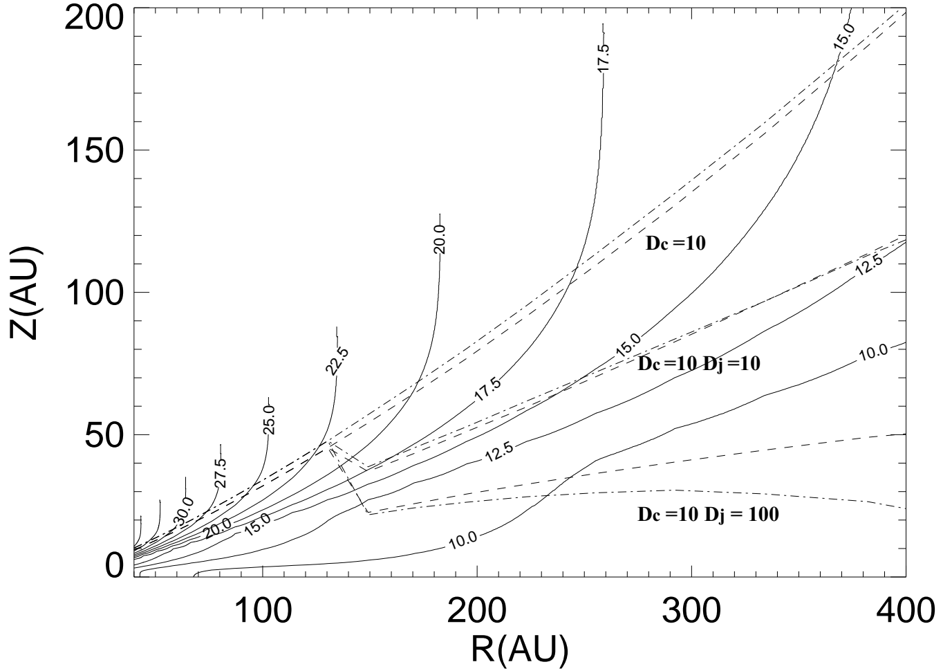
Fig. 3.— The solid contours show the gas kinetic temperature from the TW Hya model of Calvet et al. (2002). The dashed and dot-dashed lines show the \tau = 1 surfaces for the CO J=3-2 and J=2-1 lines for the three depletion scenarios described in the text.
