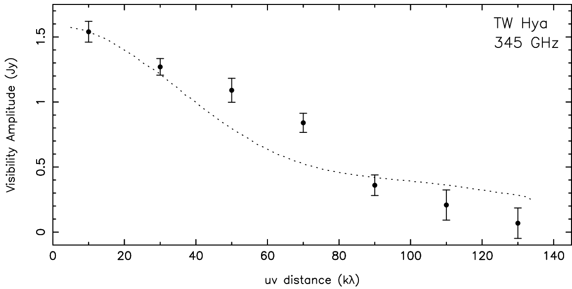
Fig. 1.— Visibility amplitudes of the observed and modeled 345 GHz continuum emission from TW Hya, annularly averaged in 20 k\lambda bins. The error bars represent \pm 1 standard deviation for each bin. The curve shows the visibility amplitudes derived from the model calculations of Calvet et al. (2002) of an irradiated accretion disk, which fits the full spectral energy distribution well after applying an amplitude scale factor of 0.9.
