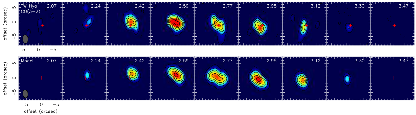
Fig. 4.— SMA images of the CO J=3–2 emission from TW Hya in 0.18 \text{ km s}^{-1} velocity bins observed with the SMA ( upper panels , with a contour spacing of 5 \text{ Jy beam}^{-1} ), together with images from a simulated observation using the model parameters listed in Table 2 ( lower panels , with a contour spacing of 3 \text{ Jy beam}^{-1} ). The small cross indicates the position of the continuum source.
