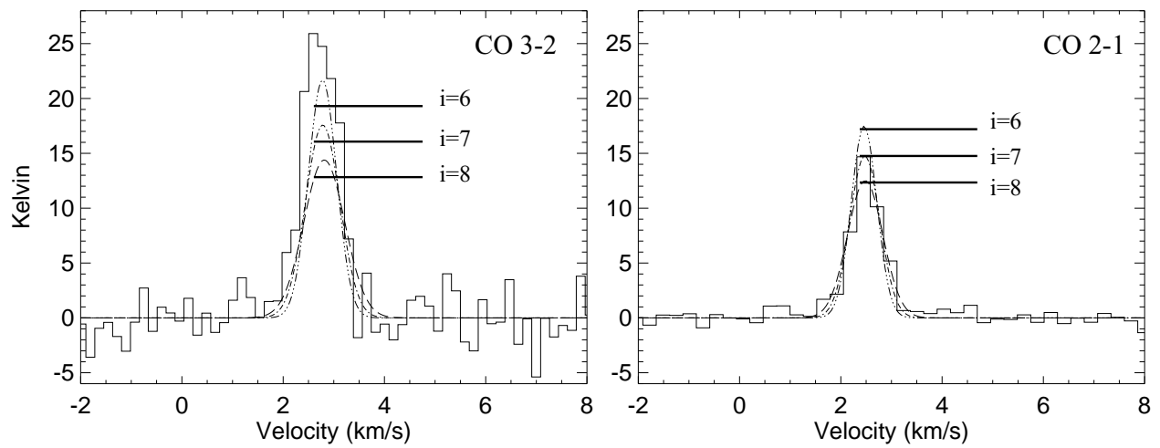
Fig. 2.— The CO J=3-2 and J=2-1 spectra at the continuum (stellar) position, beam sizes are listed in Table 1. The curves show synthetic spectra for a small range of inclination angles using the model parameters listed in Table 2.
