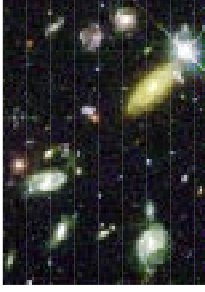
Hubble Deep Field Galaxies
