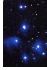
Pleiades Star Cluster
