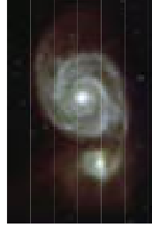
Whirlpool Galaxy
