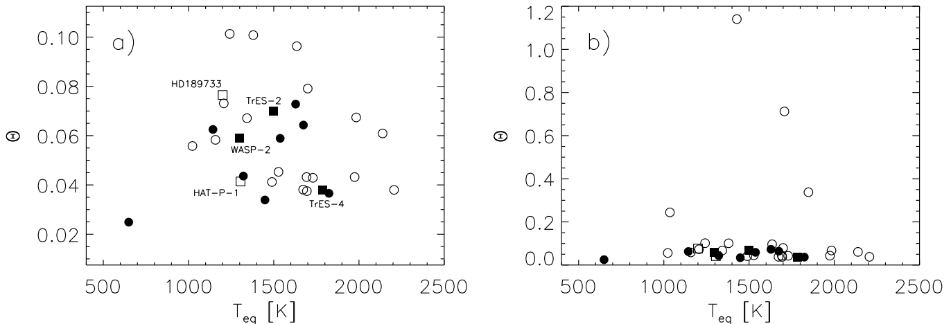
Fig. 3. a) Safronov number \Theta vs. equilibrium temperature T_{\text{eq}} for 31 transiting exoplanet systems. Circles show the position of apparently single systems, whereas squares denote known binaries. Objects marked with filled symbols have been observed in the course of the survey presented in this paper. Names in the plot identify the binary transit hosts. b) Same as a) but with a different scale for \Theta showing four additional objects with large Safronov numbers.
