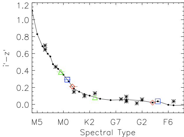
Fig. 2. i' - z' color vs. spectral type derived from template spectra from Pickles (1998) convolved with the sdss i' and z' filter curves. Overplotted are the best values for A and B component of three objects: \triangle (WASP-2), \diamond (TrES-2), and \square (TrES-4). The bars on the three leftmost items denote the spectral uncertainty of the B component of each of the three binaries, respectively. Since we assume a SpT from the literature for the A component no error bar is given. Asterisks (*) denote the positions of SDSS standard main sequence stars from Smith et al. (2002). These are included to verify the accuracy of the found relation as well as provide an uncertainty estimate of colors derived.
