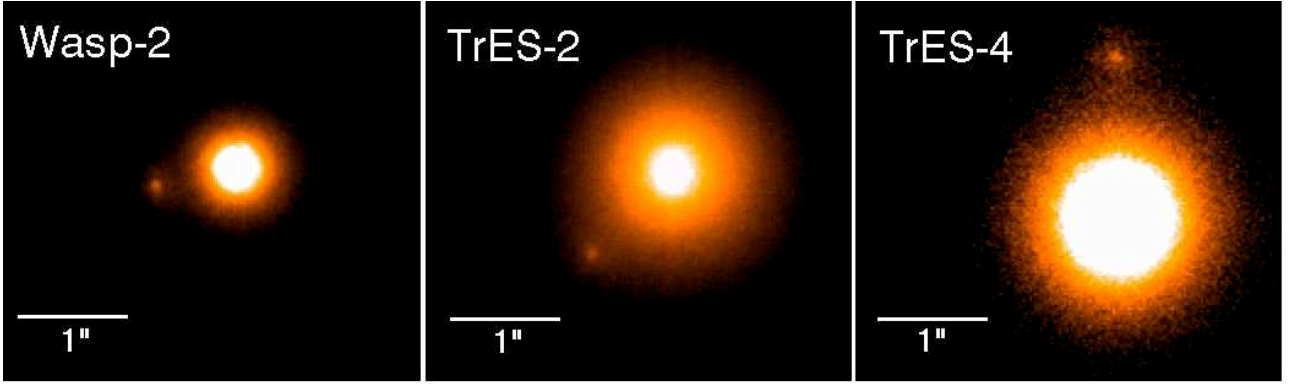
Fig. 1. z' filter images of the three exoplanet hosts with AstraLux at the Calar Alto observatory 2.2 m telescope. Total integration times are 7.68 sec for WASP-2, 15.36 sec for TrES-2, and 11.52 sec for TrES-4. The image scale is linear and cuts are adapted to best depicture the secondary. North is up and East is to the left.
