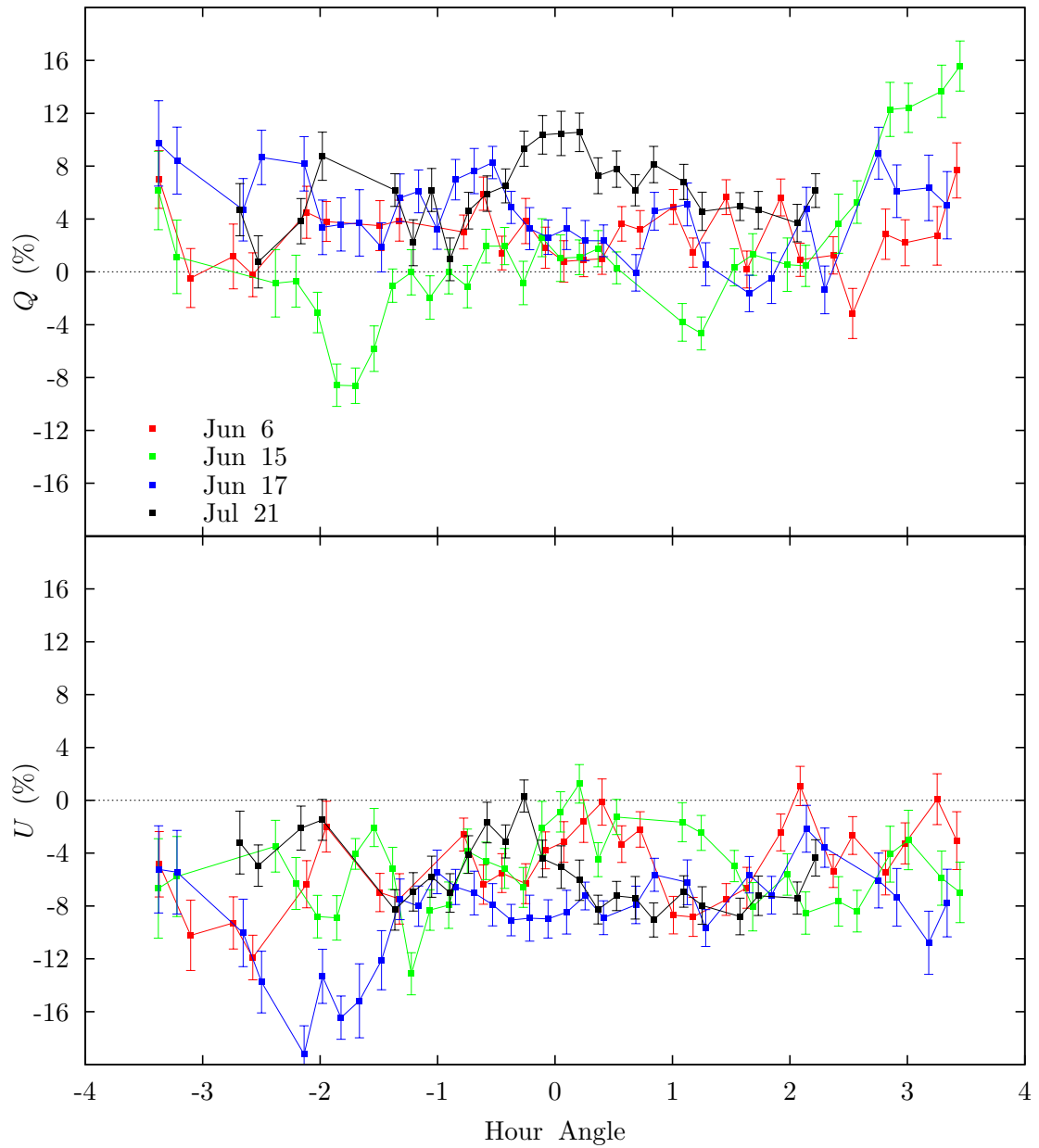
Fig. 7.14.— Like Figure 7.12, but showing the 345 GHz observations.
