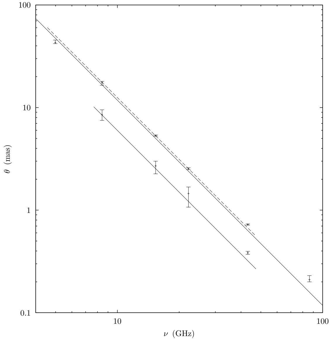
Fig. 1.2.— Angular size measurements of Sgr A* through very-long-baseline interferometry. The data points shown are taken from Shen et al. (2005). Minor axis sizes appear below major axis sizes at the frequencies where they are available. The minor axis scattering law shown is the average of the Bower et al. (2004) and Shen et al. (2005) curves, as their difference is not significant. The solid line through the major axis points uses the Bower et al. (2006) normalization for the scattering law, which is extrapolated from measurements near 1.4 GHz. The dashed curve has the Shen et al. (2005) normalization, derived from the points below 50 GHz. The intrinsic size of Sgr A* manifests itself as a deviation from the scattering law, with significant deviations visible at the highest frequencies.
