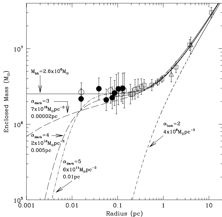
Fig. 1.1.— ( Left ): The enclosed mass as a function of projected distance from Sgr A*, based on NIR observations of stellar proper motions and radial velocities, and millimeter observations of molecular gas motions. Proper motion data are from Eckart & Genzel (1996, 1997), and Ghez et al. (1998), and are shown as open and filled circles. NIR radial velocity data from Genzel et al. (1996) are shown as open squares. The open triangles are from the millimeter data of Guesten et al. (1987). In addition to the constant mass fit (solid line), various cluster profiles described in Ghez et al. (1998) are also plotted. This figure appeared as Figure 7 in Ghez et al. (1998). ( Right ): Positions and orbital fits for seven stars in the Galactic center, Figure 2 of Ghez et al. (2005a). The positions were obtained between 1995 and 2003 using the Keck telescopes.
