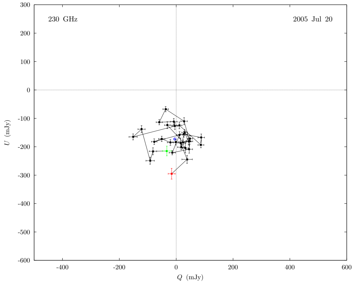
Fig. C.7.— Polarization light curve for 2005 July 20, plotted in the Q-U plane. The data are shown at full temporal resolution (one polarization switching cycle per point) as in Figure 7.7 and Table C.7. See caption of Figure C.1 for details.
