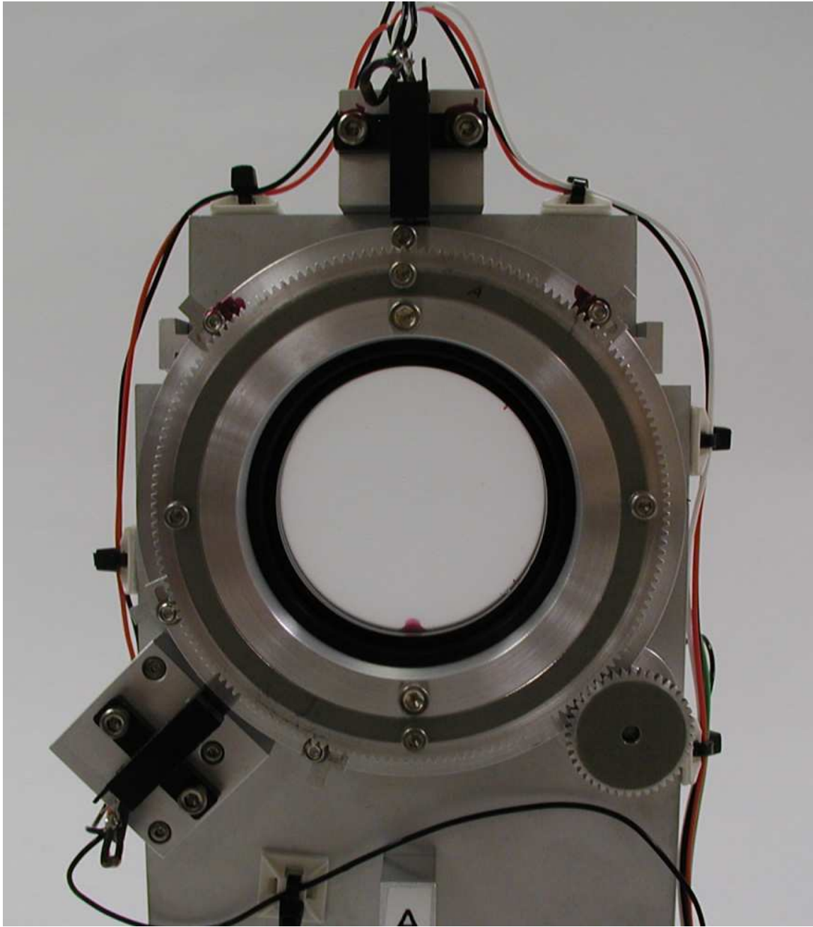
Fig. 2.6.— Closeup of the rotation stage and QWP in a wave plate positioner. Optical brakes are visible at the top and the bottom left. The adjustable flags that determine the wave plate positions are visible on the circumference of the rotation stage at \pm 45^\circ from the top and at \pm 22.5^\circ from the optical brake at the bottom left. The drive gear is visible at lower right. The alignment ring is affixed to the rear surface of the QWP.
