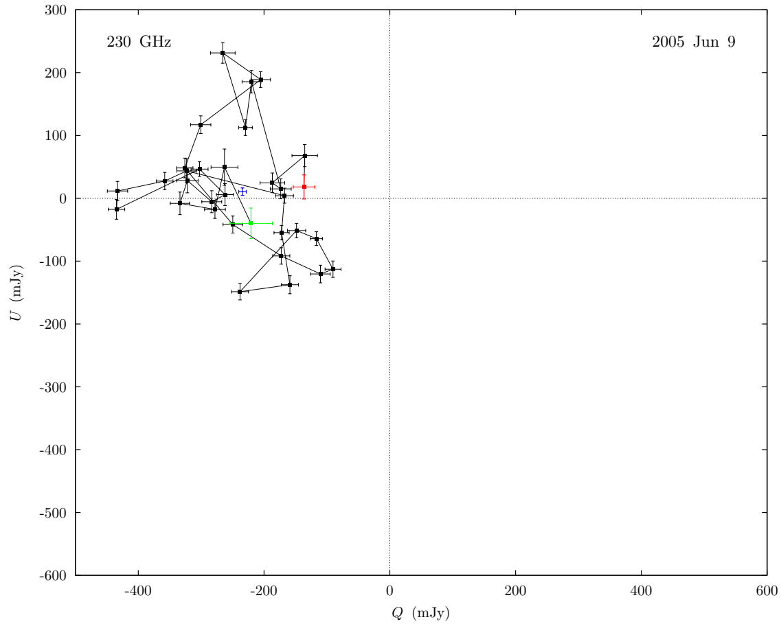
Fig. C.3.— Polarization light curve for 2005 June 9, plotted in the Q-U plane. The data are shown at full temporal resolution (one polarization switching cycle per point) as in Figure 7.3 and Table C.3. See caption of Figure C.1 for details.
