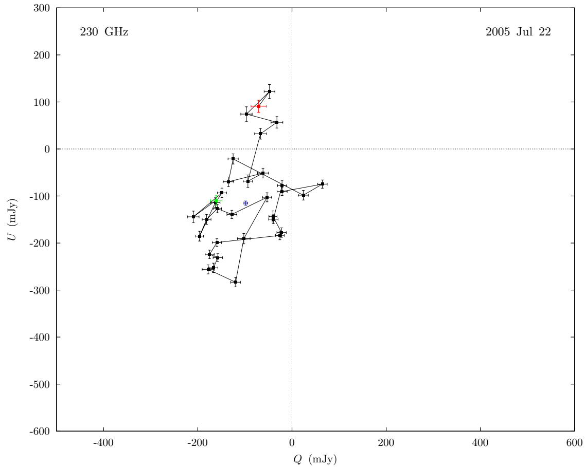
Fig. C.9.— Polarization light curve for 2005 July 22, plotted in the Q-U plane. The data are shown at full temporal resolution (one polarization switching cycle per point) as in Figure 7.9 and Table C.9. See caption of Figure C.1 for details.
