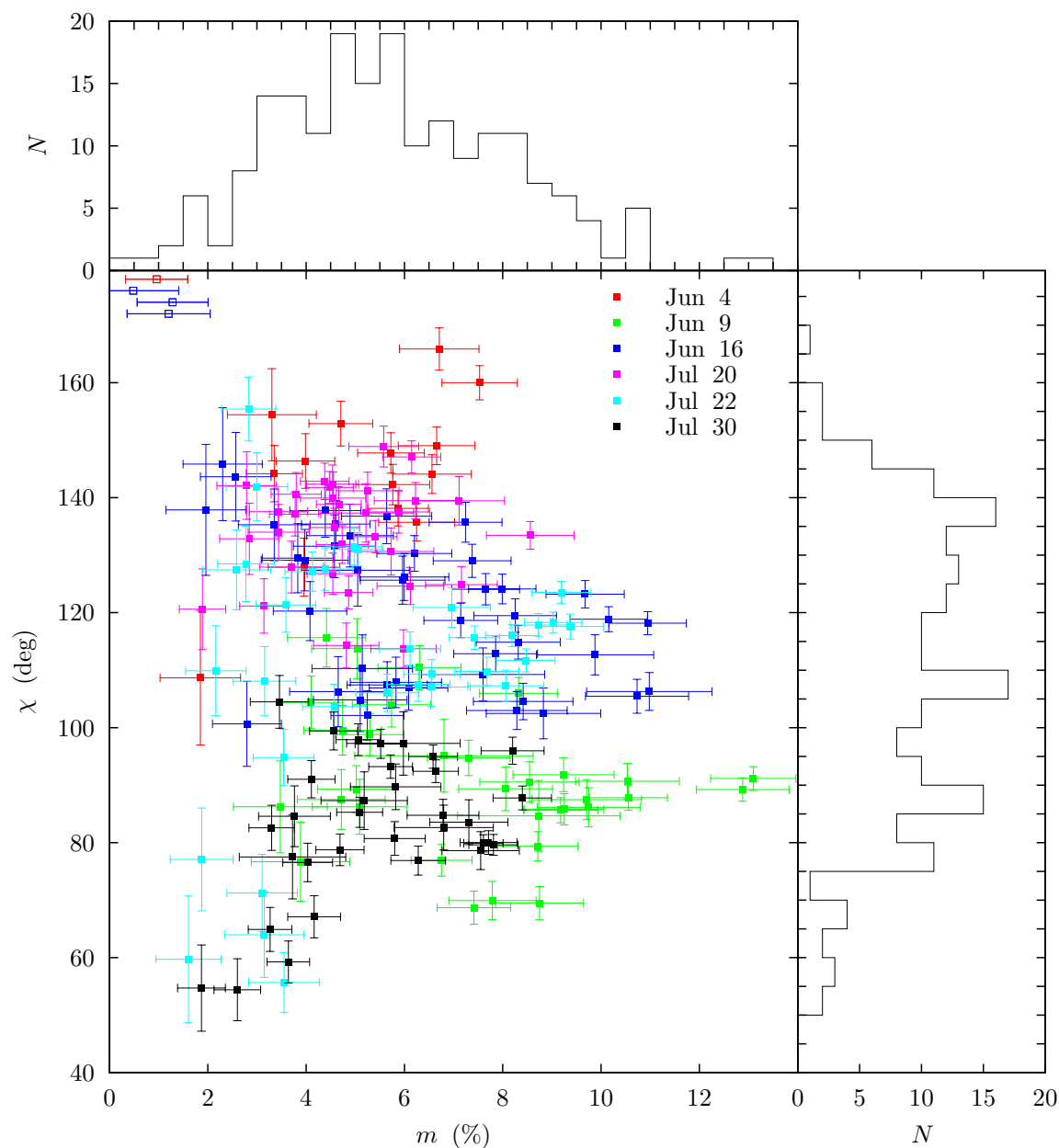
Fig. 7.15.— Short timescale polarization variability of Sgr A* at 230 GHz. Points are shown for each of the 4-minute polarization samples on six nights, 190 in all. The distribution of polarization fraction ( m ) is shown at top in 0.5% bins. The position angle ( \chi ) distribution is compiled at right with 5^\circ bins for all points where the polarization is detected at 2\sigma . The four points where the polarization falls below this threshold have very poorly constrained \chi and are shown in the upper left at arbitrary \chi .
