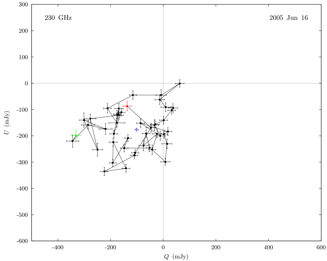
Fig. C.5.— Polarization light curve for 2005 June 16, plotted in the Q-U plane. The data are shown at full temporal resolution (one polarization switching cycle per point) as in Figure 7.5 and Table C.5. See caption of Figure C.1 for details.
