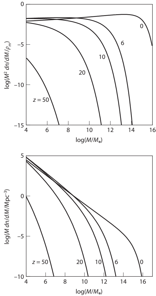
Figure 3.10 Top: The mass fraction incorporated into halos per logarithmic bin of halo mass, (M^2 dn/dM)/\rho_m , as a function of M at different redshifts z . Here \rho_m = \Omega_m \rho_c is the present-day matter density, and n(M)dM is the comoving density of halos with masses between M and M+dM . The halo mass distribution was calculated based on an improved version of the Press-Schechter formalism for ellipsoidal collapse that better fits numerical simulations (see §3.4.3). Bottom: comoving number density of halos per logarithmic bin of halo mass, Mdn/dM (in units of \text{Mpc}^{-3} ), at various redshifts.
