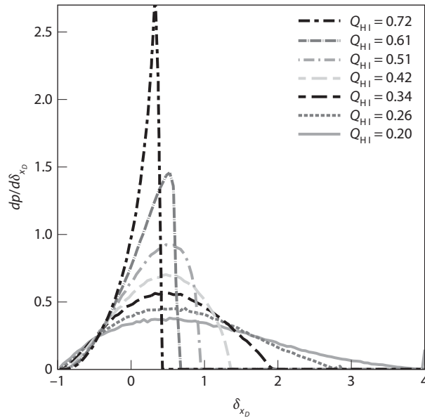
Figure 11.7 Probability distributions of the fractional bias in a simple damping wing estimate of the ionized bubble filling factor, \delta_{x_D} \equiv \bar{x}_D / (1 - Q_{H II}) - 1 . The different curves show different stages in reionization; all are computed with a seminumerical simulation of reionization. Note that the mean is always nonzero, and the distribution becomes both wider and more biased as reionization progresses. Mesinger, A., & Furlanetto, S. R., Mon. Not. R. Astron. Soc. 385 , 1348 (2008). Copyright 2008 by the Royal Astronomical Society.
