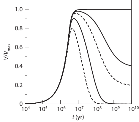
Figure 9.1 Evolution of the effective ionized volume for a stellar ionizing source, scaled to the maximum possible value V_{\max} = 4\pi\bar{n}_{\text{H}}r_{\max}^3/3 (see eq. 9.3). The solid and dashed curves assume that the sources begin shining at z = 10 and 15 , respectively. Within each set, they take C = 0, 1 , and 10 , from top to bottom. The source has \zeta = 40 and is assumed to fade with time \propto t^{-4.5} after a period t_s = 3 \times 10^6 yr, characteristic of the massive star lifetime. Reprinted from Phys. Rep. 349 , 125, Barkana, R., & Loeb, A., “In the beginning: The first sources of light and the reionization of the universe,” 125–238, Copyright 2001, with permission from Elsevier.
