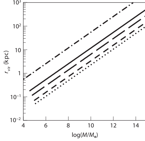
Figure 3.5 Virial radius over a wide range of halo masses and redshifts (equation 3.30). The dotted, short-dashed, long-dashed, solid, and dot-dashed curves take z = 30, 20, 10, 5, and 0, respectively.
