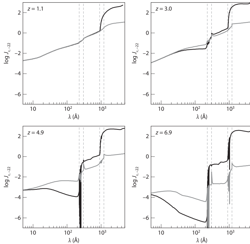
Figure 4.13 Metagalactic ionizing background spectrum at z = 1.1, 3.0, 4.9, and 6.9 , in the same theoretical model as Figure 4.8. The units correspond to J_{\nu, -22} = J_{\nu}/(10^{-22} \text{ erg cm}^{-2} \text{ s}^{-1} \text{ Hz}^{-1} \text{ sr}^{-1}) . The dark and light lines show models with galaxies and quasars, and only quasars, respectively. The vertical lines bracket the Lyman-series transitions of H I and He II. Haardt, F., & Madau, P., Astrophys. J. , 746 125 (2012). Reproduced by permission of the AAS.
