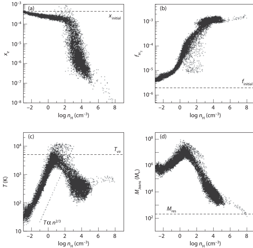
Figure 5.3 Gas properties during dense cloud collapse in a numerical simulation of first star formation. (a) Free-electron abundance; note the rapid decline at n_H \sim 10^3 \text{ cm}^{-3} , owing to efficient recombinations. (b) Molecular fraction f_{H_2} . The fraction increases rapidly during cloud collapse until the saturation value (equation 5.10) is reached, when recombinations remove the free-electron catalysts. (c) Gas temperature as a function of number density. Note the strong clump at T \sim 500 \text{ K} and n_H \sim n_{\text{cr}} , when radiative cooling becomes inefficient, so the evolution stalls. (d) The Jeans mass for this gas; note that M_J \approx 10^3 M_\odot for gas in the aforementioned stalling stage. Bromm, V., et al., Astrophys. J. 564 , 23 (2002). Reproduced by permission of the AAS.
