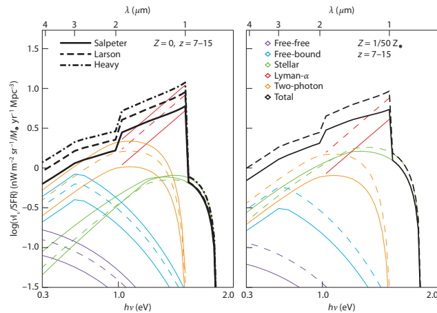
Plate 31 Near-IR background spectrum (see Figure 13.6 and associated discussion for more information). This example includes star formation in the range z = 7-15 , which dominates the background between 1 and 2 \mu\text{m} . The left panel assumes metal-free stars, while the right panel takes a metallicity Z = 0.02 Z_{\odot} . The different line styles show different IMFs (see text). The different curves show the total emission, the Lyman- \alpha contribution, the stellar continua, the two-photon continua, the free-bound emission, and finally the free-free emission (from top to bottom at 1 \mu\text{m} ). Fernandez, E. R., & Komatsu, E., Astrophys. J. 646 , 703 (2006). Reproduced by permission of the AAS.
