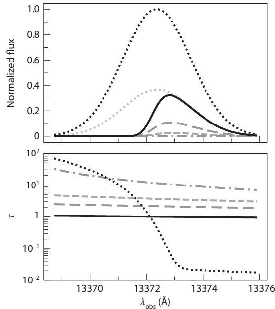
Figure 11.13 Top : Example line profiles for a galaxy at z = 10 . The upper dotted curve shows the intrinsic line profile, assumed to be a Gaussian with standard deviation 27 \text{ km s}^{-1} . The solid, long-dashed, and short-dashed curves show the observed line after reprocessing through the IGM; they place the galaxy in ionized bubbles with radii R_b = 10, 5, and 3 comoving Mpc, respectively. The lower dotted curve shows the line if we neglect resonant absorption within the ionized bubble, assuming R_b = 10 Mpc. Bottom : The dotted line shows the resonant absorption from the ionized bubble. The solid, long-dashed, short-dashed, and dot-dashed curves show the damping wing optical depth for R_b = 10, 5, 3, and 1 Mpc, respectively. Furlanetto, S. R., et al., Mon. Not. R. Astron. Soc. 354 , 695 (2004). Copyright 2004 by the Royal Astronomical Society.
