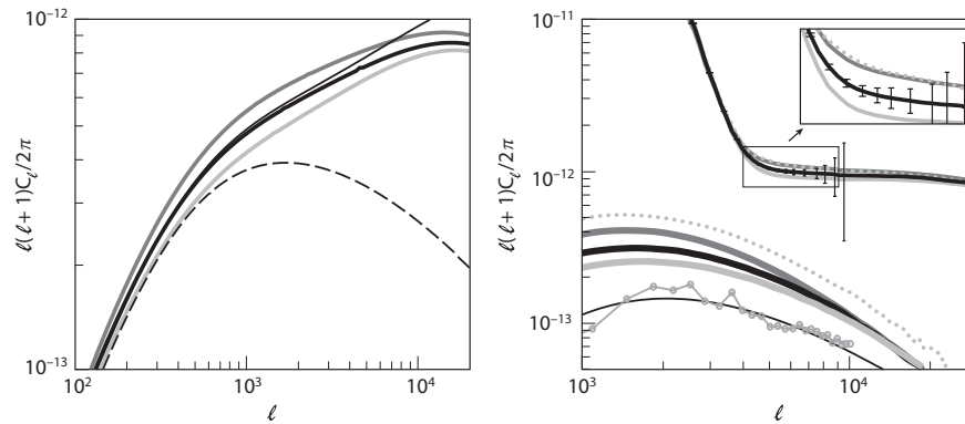
Figure 13.5 Left : Angular power spectrum of the Ostriker-Vishniac effect on the CMB. The thick, solid curves take models in which reionization ends at z_{\text{reion}} = 8, 12, and 18, from bottom to top. The thin solid curve shows the signal without any baryonic filtering, while the thin dashed curve shows the signal assuming only a linear theory density field. Right : The patchy reionization signal from the same models (lower left, thick curves) and the total CMB anisotropy power spectrum (at upper right, including the primordial, lensing, and Ostriker-Vishniac components as well); note the change in the scale of the vertical axis on this panel. In addition, the dotted curve shows the patchy signal from a model with extended reionization. The open circles show the estimate from a seminumerical simulation of reionization, with the thin line a corresponding analytic estimate with the same reionization history; the two match very well. The error bars at upper right are representative of existing instruments, assuming perfect foreground removal. McQuinn, M., et al., Astrophys. J. 630 , 643 (2005). Reproduced by permission of the AAS.
