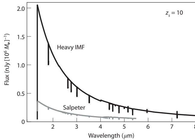
Figure 5.14 Comparison of the observed flux per unit frequency from a cluster of Population III stars at a redshift z_s = 10 for a Salpeter IMF ( light line ) and an IMF composed purely of very massive stars ( dark line ). The cutoff below an observed wavelength of 1216 \text{ \AA} (1 + z_s) = 1.34 \mu\text{m} is due to hydrogen Lyman- \alpha absorption in the IGM (the so-called Gunn-Peterson effect; see §4.3). Bromm, V., Kudritzki, R. P., & Loeb, A., Astrophys. J. 552 , 464 (2001); Salpeter curve from Tumlinson, J., & Shull, M. J., Astrophys. J. 528 , L65 (2000). Reproduced by permission of the AAS.
