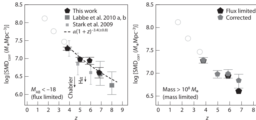
Figure 10.12 Stellar mass density (SMD) evolution over redshift in galaxies brighter than M_{\text{AB}} = -18 at a rest-frame wavelength of 1500 \text{ \AA} ( left ) and with stellar mass M_{\star} > 10^8 M_{\odot} ( right ) from several different measurements. All panels assume a Salpeter IMF and Z = 0.2 Z_{\odot} ; the line labeled “Chabrier” shows the effect of assuming a different IMF. The other line (labeled “H \alpha ”) shows the effect of systematic contamination from line emission. Gonzalez, V., et al., Astrophys. J. 735, L34 (2011). Reproduced by permission of the AAS.
