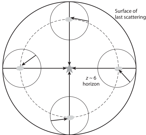
Figure 13.1 Diagram of the damping of primordial CMB anisotropies after reionization (not to scale). The observer is represented by the star at the center; the thick outer circle represents the surface of last scattering of the observer. CMB photons (arrows) propagate through a screen of parcels of free electrons at z \sim 6 (located at the dashed circle for the observer). Each parcel sees the CMB out to its causal horizon, represented by the smaller circle surrounding it. The low optical depth of free electrons implies that most CMB photons propagate through without interaction (long arrows), but some photons are scattered into the line of sight from other directions, which partially washes out the primordial anisotropies on scales smaller than the horizon at the time of scattering.
