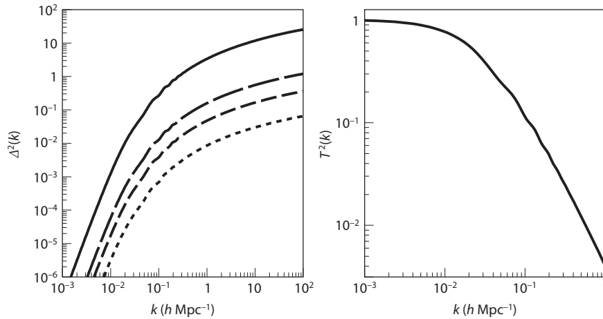
Figure 2.1 Left : The matter power spectrum in our fiducial cosmology at z = 0, 5, 10, and 25 , from top to bottom. Right : The corresponding transfer function. Computed using the publicly available code CAMB ( http://camb.info ).
