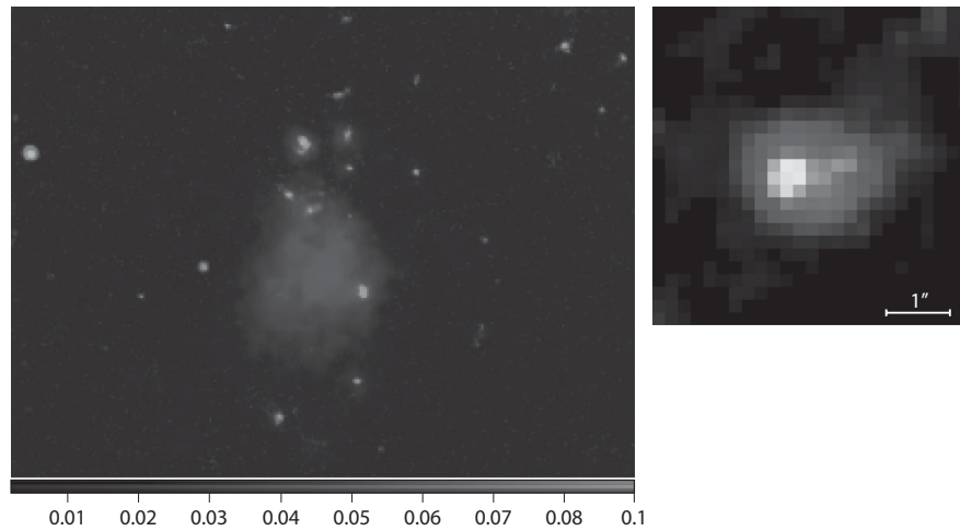
Figure 11.12 Left : A false-color image of a Lyman- \alpha blob (LAB) at redshift z = 2.656 . The hydrogen Lyman- \alpha emission is shown together with the images in the optical V-band and the near-IR J and H bands. (See Color Plate 25 for a color version of this figure.) Note the compact galaxies lying near the northern (top) end of the LAB. The Lyman- \alpha image was obtained using the SuprimeCam imaging camera on the Subaru Telescope, and the V, J, and H band images were obtained using the ACS and NICMOS cameras on the Hubble Space Telescope. This LAB was originally discovered by the Spitzer Space Telescope. Prescott, M., & Dey, A. (2010). Right : A false-color image of a LAB at redshift z = 6.6 , obtained from a combination of images at different IR wavelengths. Ouchi, M., et al., Astrophys. J. 696 , 1164 (2009). Reproduced by permission of the AAS.
