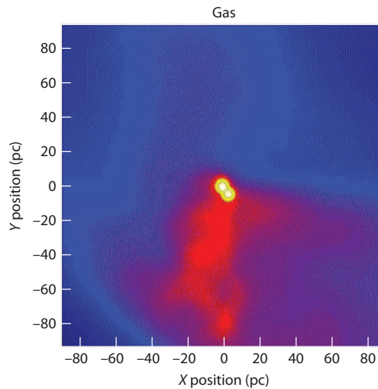
Plate 14 Numerical simulation of the collapse of an early dwarf galaxy with a virial temperature just above the cooling threshold of atomic hydrogen and no \text{H}_2 (see Figure 7.6 and associated discussion for more information). The image shows a snapshot of the gas density distribution 500 million years after the Big Bang, indicating the formation of two compact objects near the center of the galaxy with masses of 2.2 \times 10^6 M_\odot and 3.1 \times 10^6 M_\odot , respectively, and radii < 1 pc. Sub-fragmentation into lower mass clumps is inhibited because hydrogen atoms cannot cool the gas significantly below its initial temperature. These circumstances lead to the formation of supermassive stars that inevitably collapse to make massive seeds for supermassive black holes. The simulated box size is 200 pc on a side. Bromm, V., & Loeb, A., Astrophys. J. 596 , 34 (2003). Reproduced by permission of the AAS.
