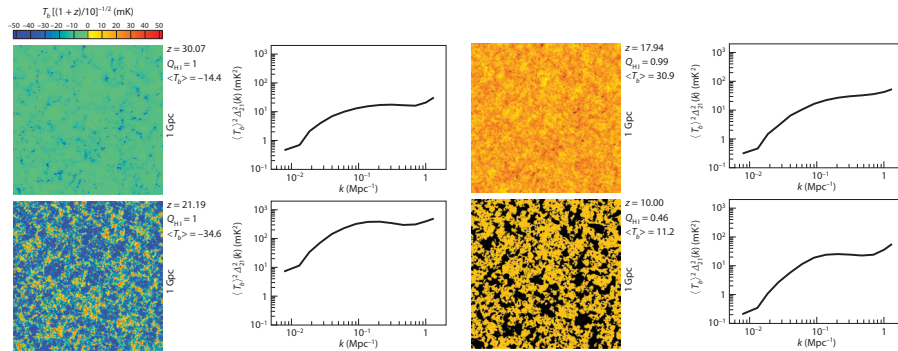
Plate 29 Slices through a “seminumerical” simulation ( left ), and the corresponding spherically averaged power spectra ( right ), for a model of the spin-flip background at z = 30.1 , 21.2, 17.9, 10.0 ( top to bottom ; see Figure 12.14 and associated discussion for more information). The slices were chosen to highlight various epochs in the cosmic 21-cm signal (from top to bottom): the onset of Lyman- \alpha pumping (here the blue regions show the cold gas around the first galaxies); the onset of X-ray heating (here the blue regions are cold gas, while the compact red regions represent hot gas around the first black holes); the completion of X-ray heating (where all the gas is hot); and the midpoint of reionization (where black regions are ionized bubbles). All slices are 1 Gpc on a side and 3.3 Mpc deep. Mesinger, A., Furlanetto, S. R., & Cen, R., Mon. Not. R. Astron. Soc. 411 , 955 (2011). Copyright 2011 by the Royal Astronomical Society.
