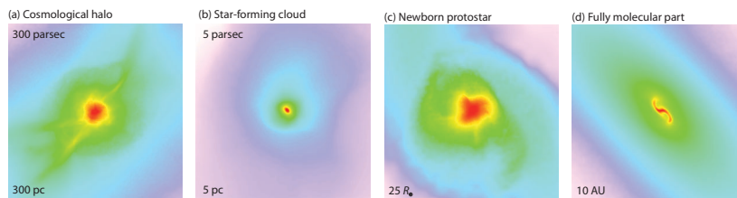
Plate 4 Projected gas distribution around a primordial protostar from a numerical simulation (see Figure 5.6 and associated discussion for more information). Shown is the gas density of a single object on different spatial scales: (a) the large-scale gas distribution around the cosmological mini-halo; (b) the self-gravitating, star-forming cloud; (c) the central part of the fully molecular core; and (d) the final protostar. Reprinted from Science , 321 , 5889, Yoshida, N., K. Omukai, & L. Hernquist, "Protostar Formation in the Early Universe," Copyright 2008, with the permission of the American Association for the Advancement of Science.
