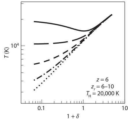
Figure 9.13 IGM temperature–density relation following H I reionization. All curves assume z = 6 and take a postreionization temperature of T_{\text{H}} = 20,000 K. The solid, long-dashed, short-dashed, dot-dashed, and dotted curves set the reionization redshift at z_r = 6, 7, 8, 9, and 10 , respectively. Furlanetto, S. R., & Oh, S. P., Astrophys. J. 701 , 94 (2009). Reproduced by permission of the AAS.
