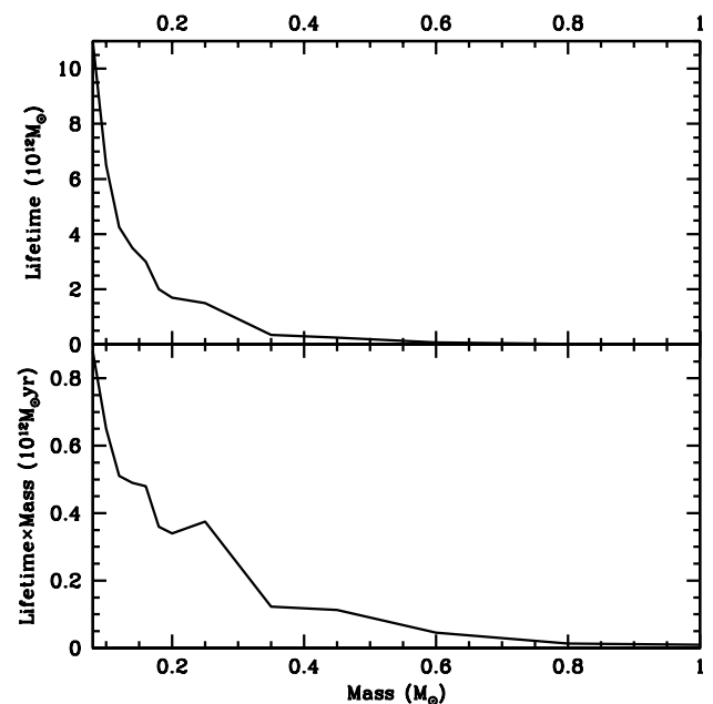
FIG. 1: The dependence of the lifetime of low-mass stars on their mass. The upper panel shows the lifetime and the lower-panel shows the product of the lifetimes with the stellar mass.
