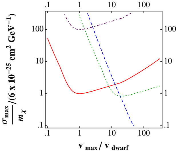
FIG. 2: Astrophysical constraints on the normalization of the self-interaction cross-section ( \sigma_{\max} ) as a function of the velocity at which the peak collision rate is obtained ( v_{\sigma} ) in Fig. 1. The red solid line is normalized to have \langle\sigma\rangle_{\max}/m_{\chi} \approx 6 \times 10^{-25} \text{ cm}^2/\text{GeV} at v_{\text{dwarf}} \approx 10 \text{ km s}^{-1} , which should be regarded as the minimum interaction necessary to flatten the cores of dwarf galaxies. Additional lines indicate upper limits on the cross-section based on astrophysical considerations: X-ray cluster ellipticity ( blue, dashed ), limiting (\sigma_{\max}/m_{\chi}) \lesssim 4 \times 10^{-26} \text{ cm}^2/\text{GeV} at v \sim 10^3 \text{ km s}^{-1} ; destruction of dwarf sub-halos through collisions with high velocity particles from a larger parent halo in which these dwarfs are embedded ( green, dotted ), limiting (\sigma_{\max}/m_{\chi}) \lesssim 5 \times 10^{-25} \text{ cm}^2/\text{GeV} [?] at v \sim 200 \text{ km s}^{-1} ; and requiring the number of scatters in dwarfs to be less than \sim 10^2 during the age of the Universe to avoid the gravothermal catastrophe ( purple, dash-dotted ).
