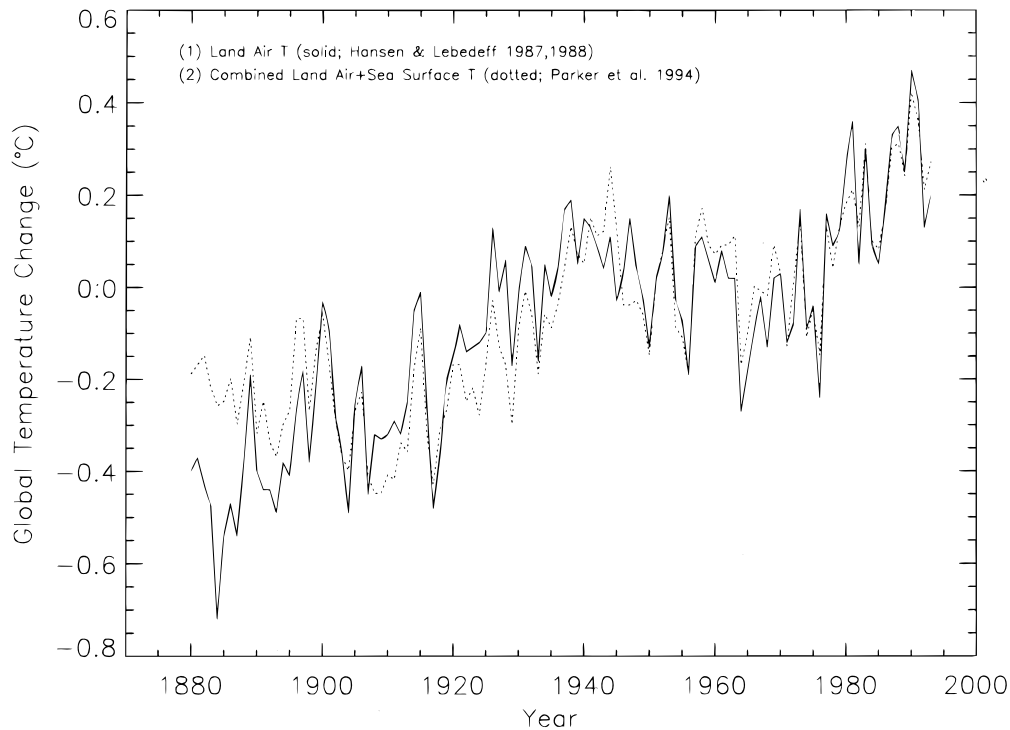
FIG. 2.—Annual average, global land-air surface temperature anomalies (relative to the 1951–1980 reference) derived by Hansen & Lebedeff (1987, 1988; solid curve ), and the combined land-air and sea surface temperature record of Parker et al. (1994; dotted curve ). Except for the data prior to 1890, the close concordance of the two reconstructions suggests that the long-term trend of global terrestrial surface temperature changes used in the present study is robust. Spatial coverage of historical temperature series prior to the 1850s to 1860s is poor, and therefore those periods are not considered in this study.
