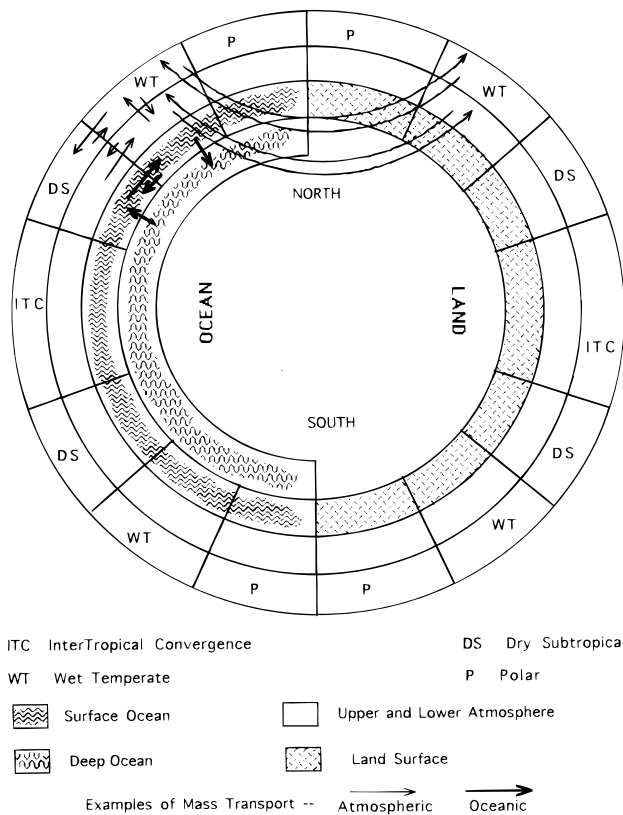
FIG. 1.—Geometry of the energy-balance climate model
